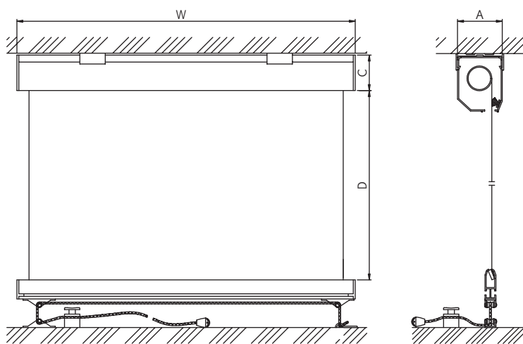
DIMENSION TABLE
